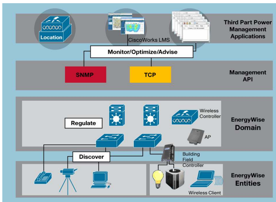
Figure 4. Cisco EnergyWise Intelligent Network Framework
