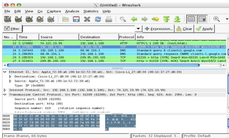
Figure 2. Wireshark GUI
